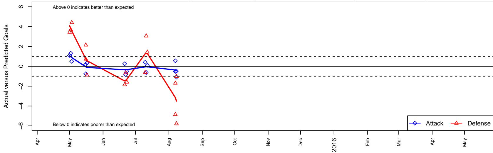
Spokane Foxes Premier G98 Dots are actual minus expected GF (blue circles) and GA (red triangles). Blue line is smoothed change in attack strength. Red is smoothed change in defense strength.
